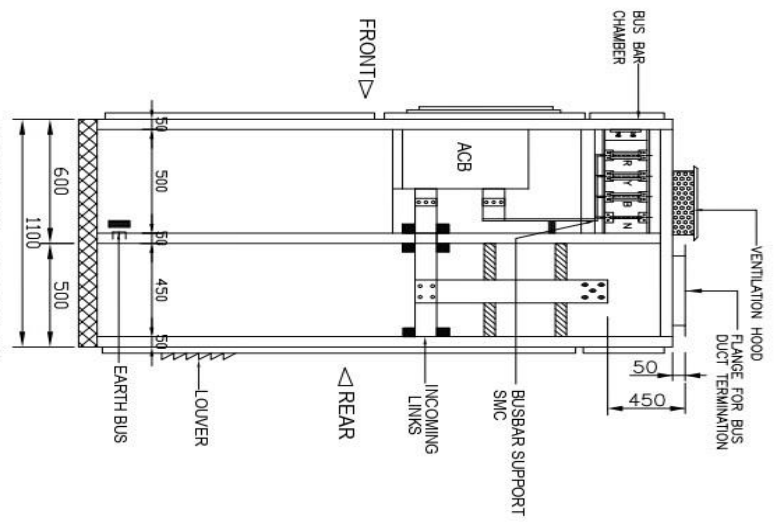
SECTIONAL SIDE VIEW TYP. BUS BAR ARRANGEMENT
