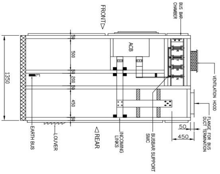
SECTIONAL SIDE VIEW TYP. BUS BAR ARRANGEMENT
